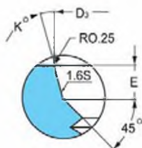
Detail X
